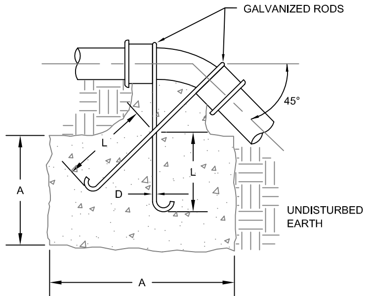
VERTICAL BLOCKING FOR 45° BENDS
